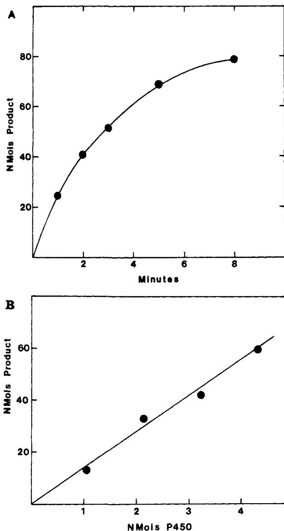
Figure 1. Hydroxylation of cyclohexane by 1 and cytochrome P-450. The concentration of cyclohexane was 10 mM. Other conditions were as in the Experimental Section. (A) Accumulation of cyclohexanol as a function of time. The concentration of P-450 LM2 was 3.6 \mu M and the concentration of 1 was 2 mM. (B) Total nmol of cyclohexanol accumulated after a 2-min reaction period as a function of P-450 concentration. The concentration of 1 was 4 mM.
